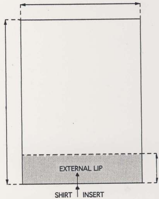
BAG WITH INTERNAL WELDED LIP
